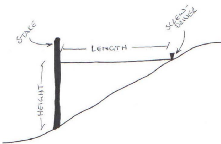
Figure 4: Set-up diagram with length and height marked
